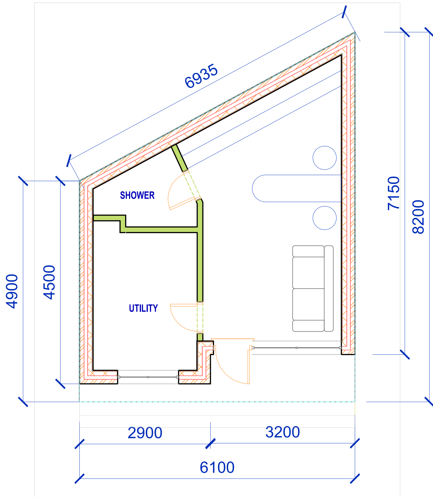
GROUND FLOOR PLAN - EXISTING 1:50 (PROPOSED FOR RETENTION)
