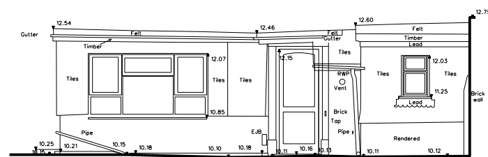
ELEVATION 5 - WEST
