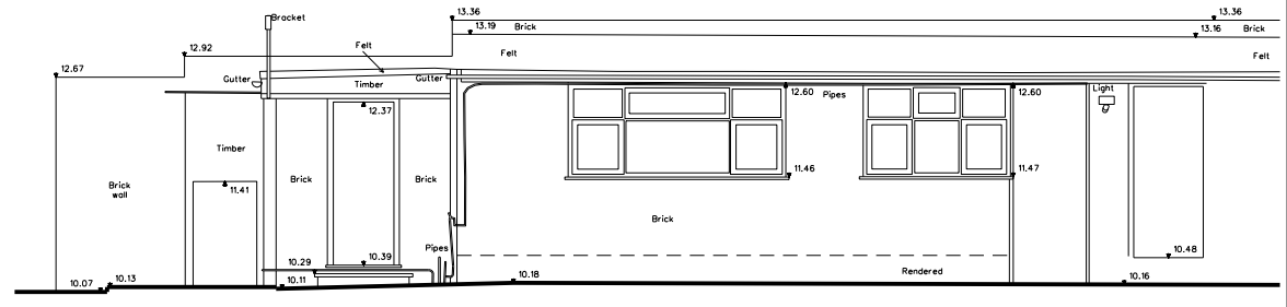
ELEVATION 2 - EAST
