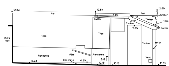
ELEVATION 6 - NORTH
