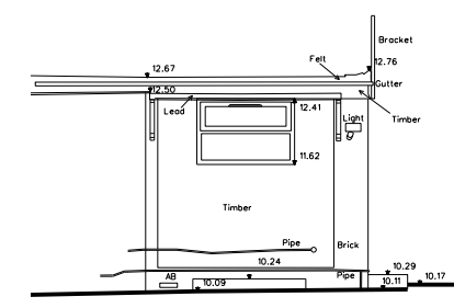
ELEVATION 1 - SOUTH
