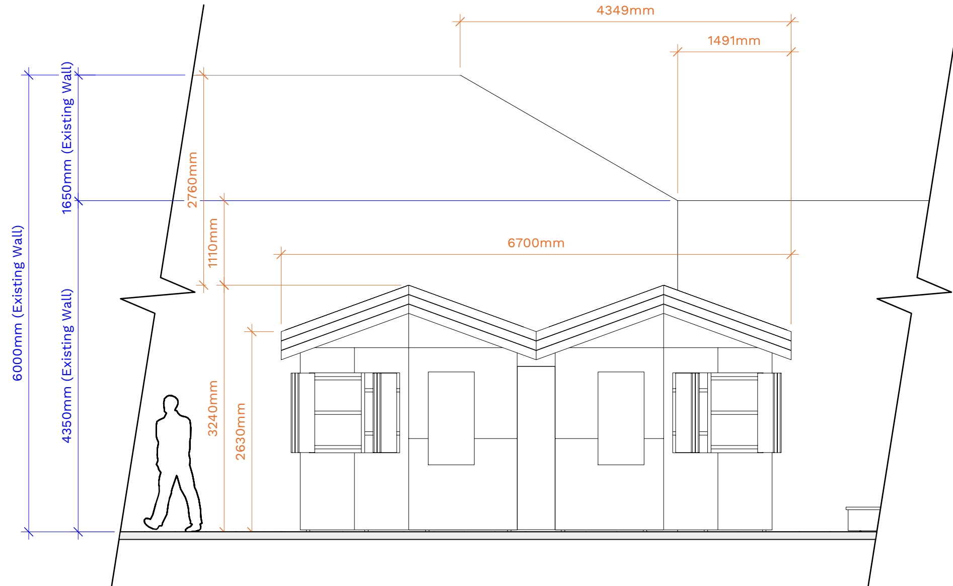
2 Elevation of Detail A (Ref 01.1) Scale: 1:50
