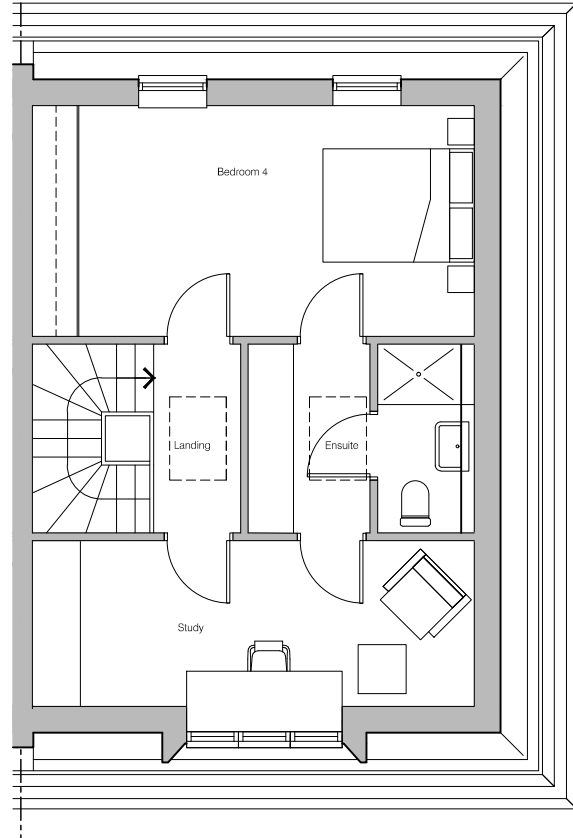
07 Third Floor Plan 1:50 @ A1 / 1:100 @ A3
