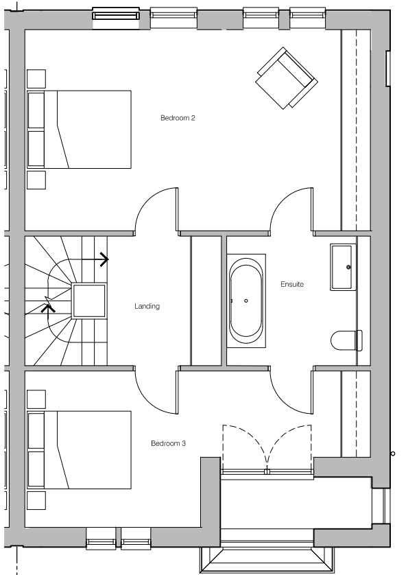
03 Second Floor Plan 1:50 @ A1 / 1:100 @ A3
