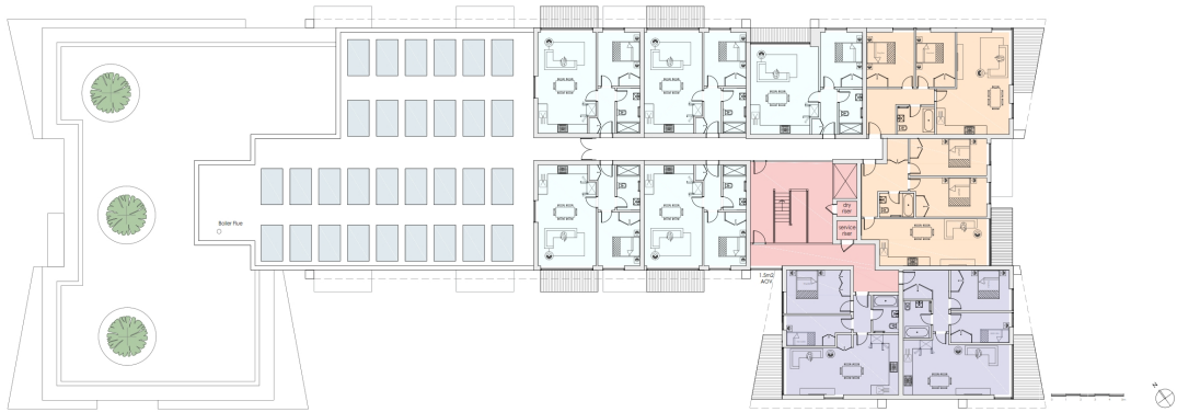
PROPOSED 5TH FLOOR PLAN
